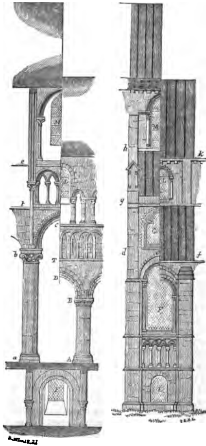
71. Canterbury Cathedral.
